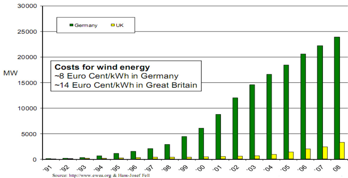
Figure 1: Wind power development in the UK and Germany 1992-2008 xlv
